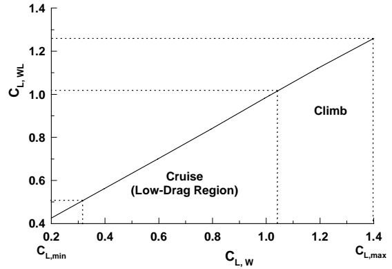
Fig. 1 Winglet lift-coefficient operating range compared to that of the wing for a typical high-performance sailplane.
