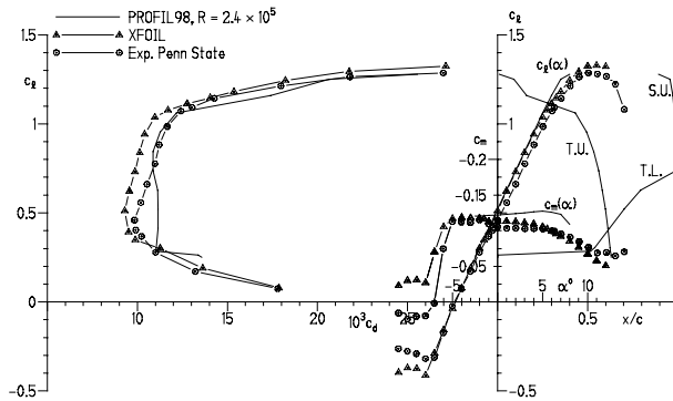
Fig. 11 Comparison of theoretical and experimental section characteristics for R = 2.4 \times 10^5 .
