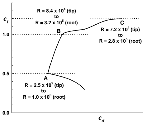
Fig. 3 Summary of design requirements for airfoil.
